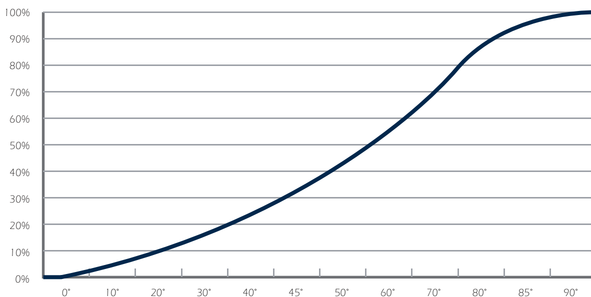
Cv curve %
