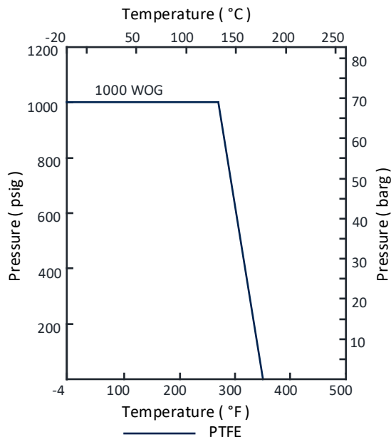
Valve Body Rating with Seat Material Plot :
