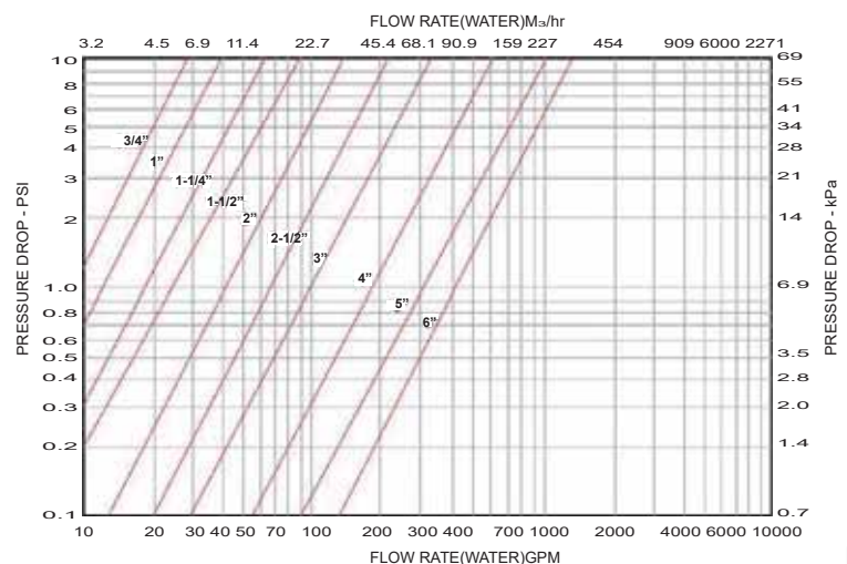
Curve of pressure drop & flowrate
